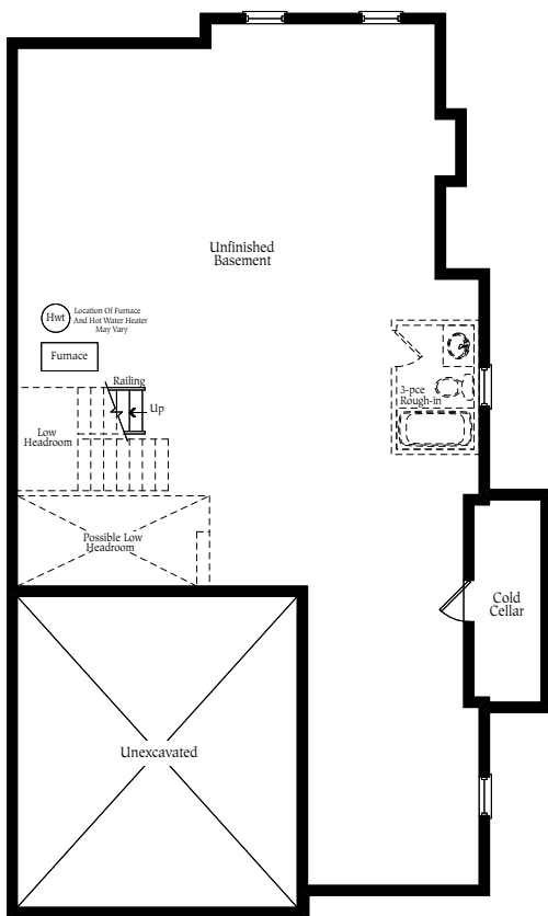
Basement Elevation A & C
