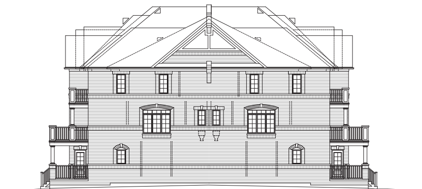
BLOCK 3 RIGHT SIDE ELEVATION
