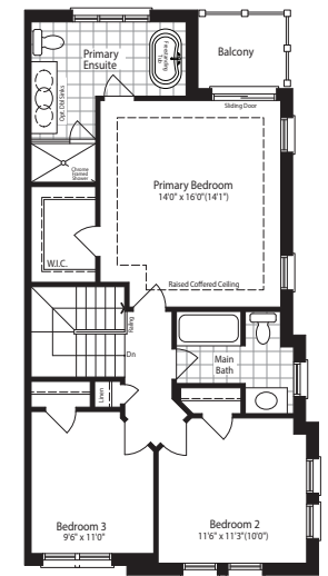
SECOND FLOOR Elevation A Upgrade (Lot 16 only)
