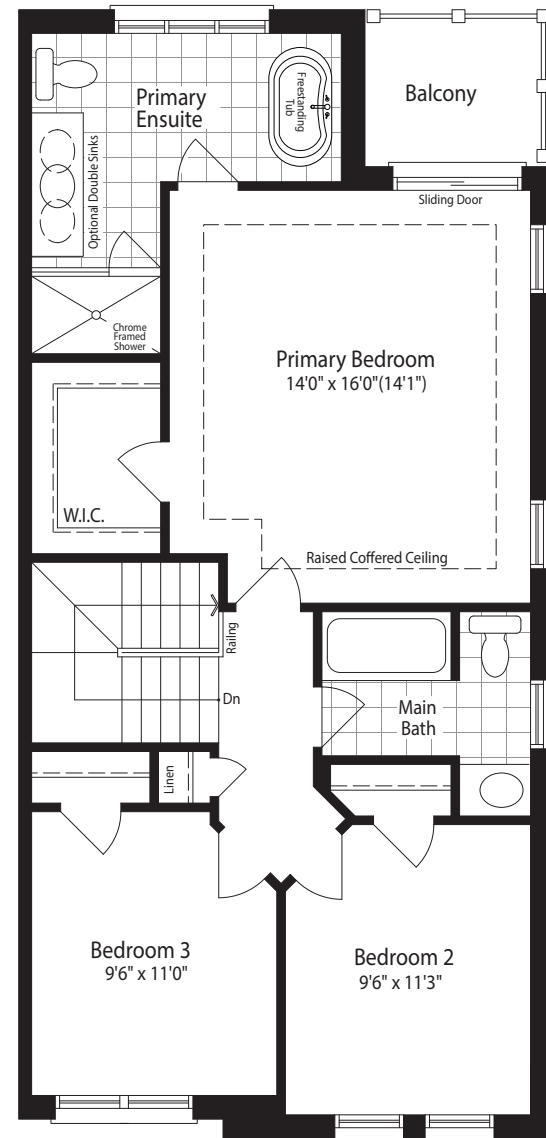
SECOND FLOOR Elevation A
