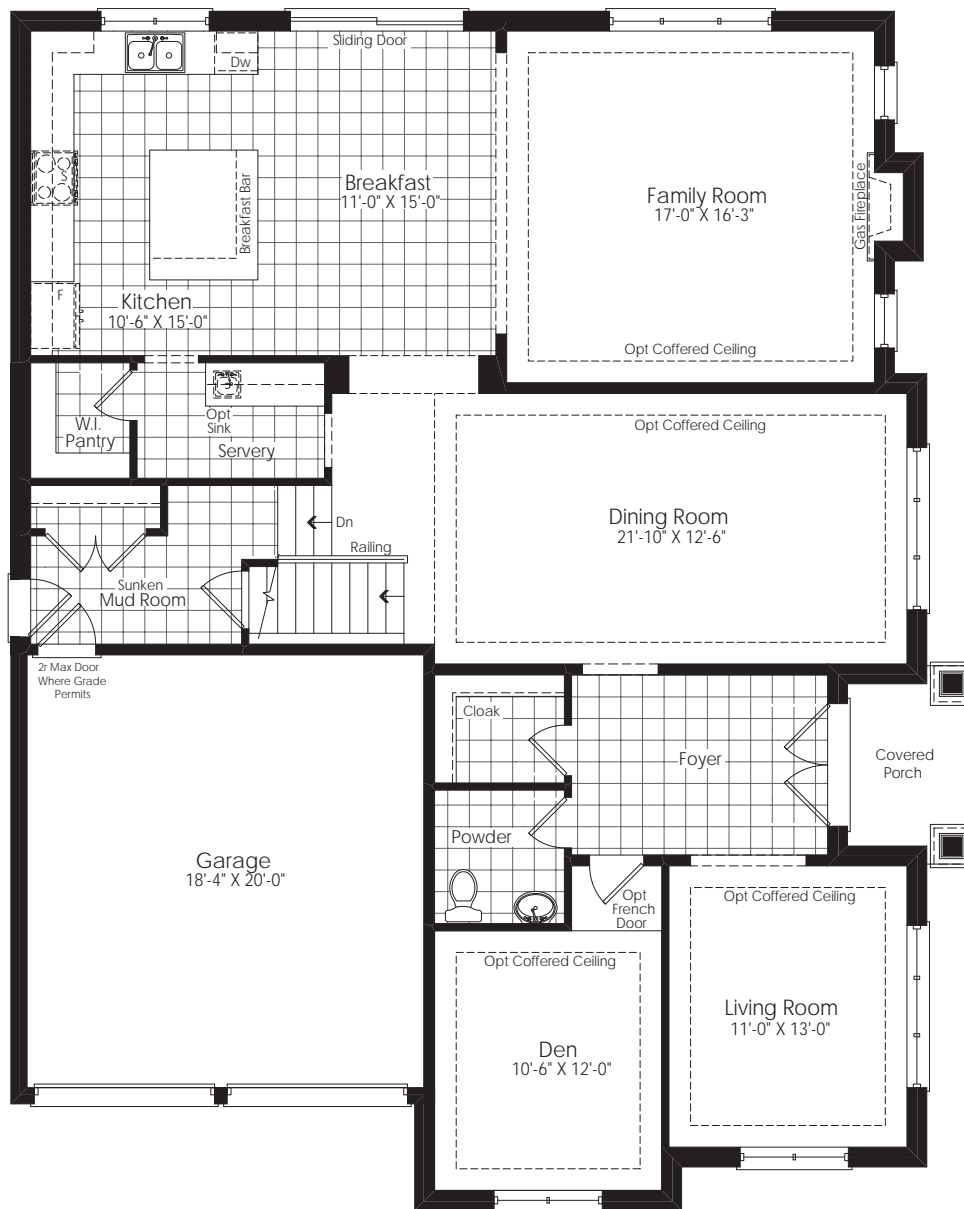
Ground Floor Elevation A & B
